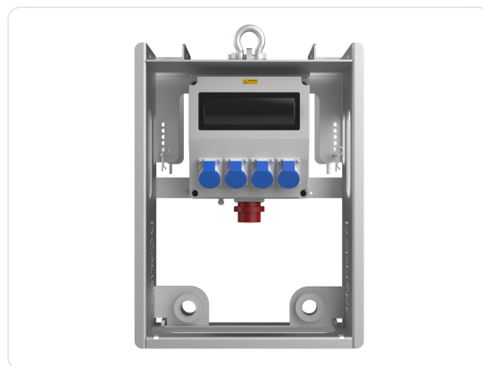
The distribution frame: four outlets to the luminaires and one supply inlet.
